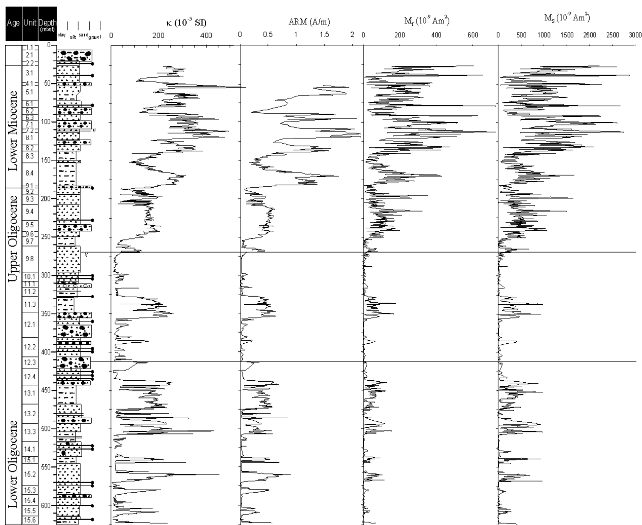
Fig. 1 – Down-core variation of ferrimagnetic concentration-dependent parameters ( k , ARM, M_r and M_s ) in CRP-2/2A. The lines at 270 and 413 mbsf indicate the boundaries between intervals with different magnetic properties (see discussion in text, Fig. 2 & Tab. 1).
