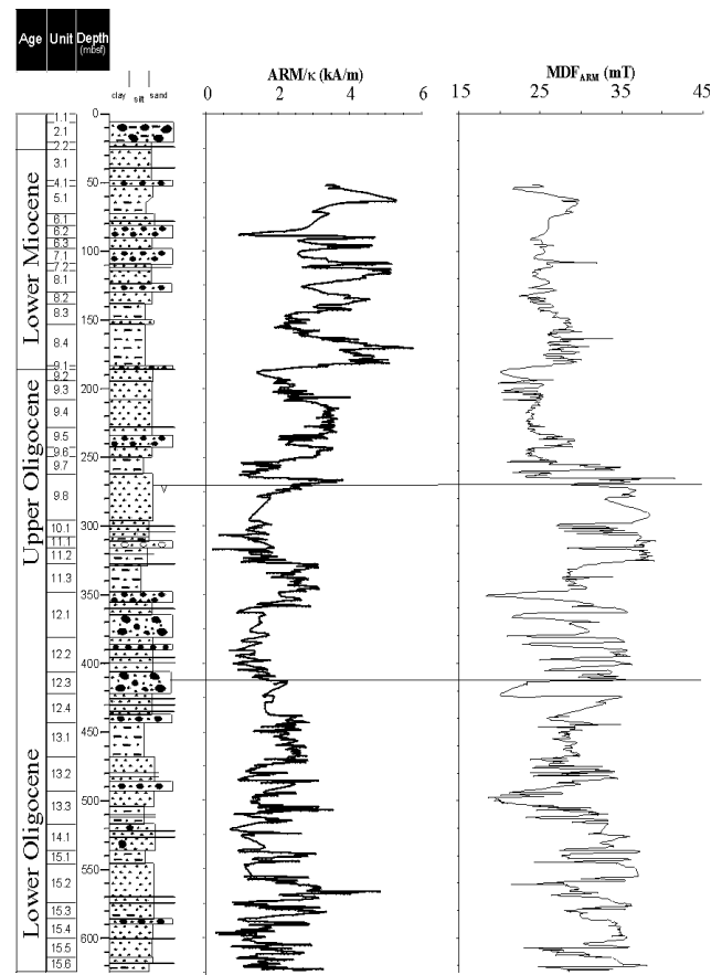
Fig. 5 – Down-core variations of ARM/k and MDF_{ARM} for CRP-2/2A. The lines at 270 and 413 mbsf indicate the boundaries between intervals with different magnetic properties.
