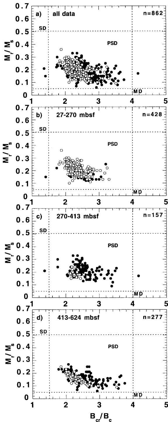
Fig. 4 – Plots of M_r/M_s versus B_{cr}/B_c for: a) all data from CRP-2/2A, b) the interval between 27 and 270 mbsf, c) the interval between 270 and 413 mbsf, and d) the interval between 413 and 624 mbsf. Open symbols correspond to points with high magnetic mineral concentration; closed symbols correspond to points with low magnetic mineral concentration. The fields marked for SD = single-domain, PSD = pseudo-single-domain, and MD = multi-domain, correspond to the ranges of values expected for crushed (titano)magnetite grains (Day et al., 1977).
