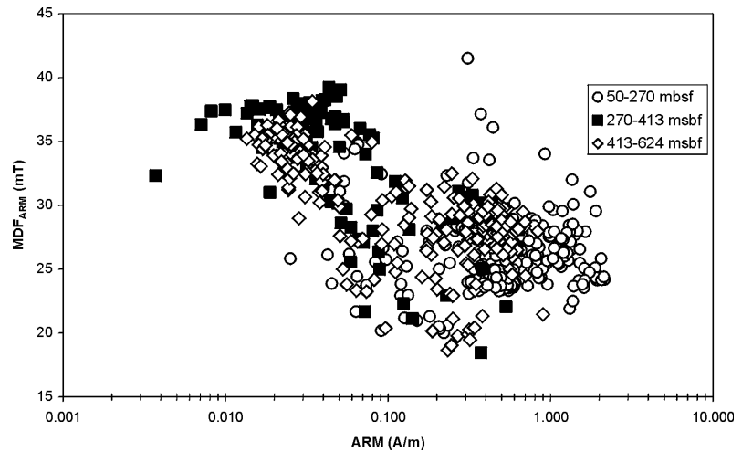
Fig. 7 – Plots of MDF_{ARM} versus ARM for all data from CRP-2/2A. Two clusters of samples can be distinguished: one with low ARM intensities and relatively high MDF_{ARM} values corresponds to hematite-enriched samples; the other with high ARM intensities and low MDF_{ARM} values corresponds to magnetite-enriched samples. The points scattered between these clusters represent samples with a mixture of magnetite and hematite.
