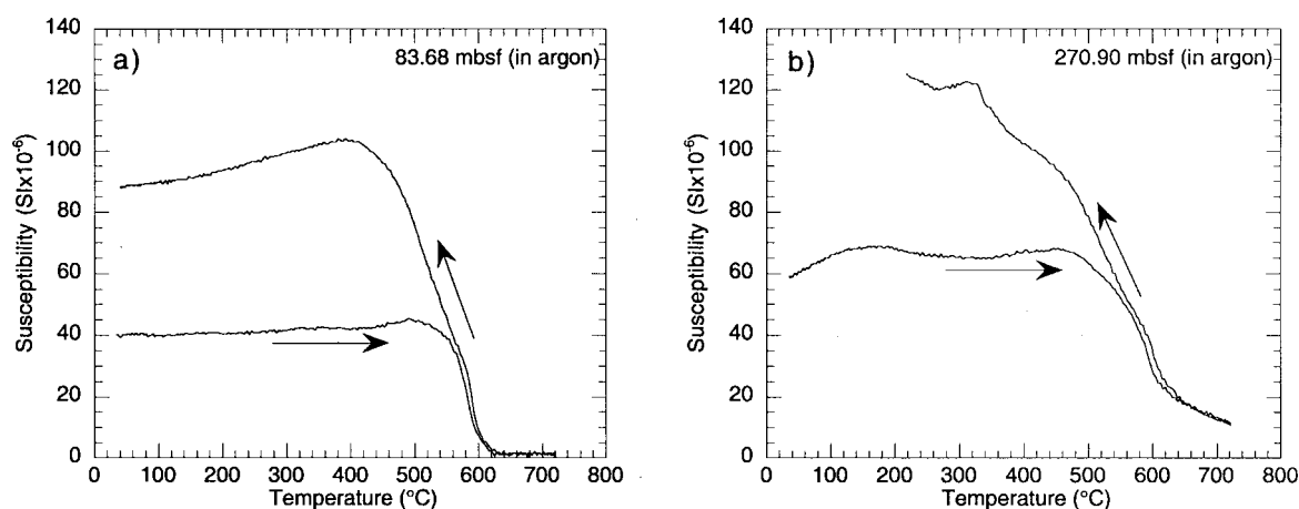
Fig. 3 – Temperature-dependent susceptibility plots for two representative samples: a) 83.68 mbsf, which is dominated by magnetite, and b) 270.90 mbsf, which contains evidence for a mixture of magnetite and hematite.
