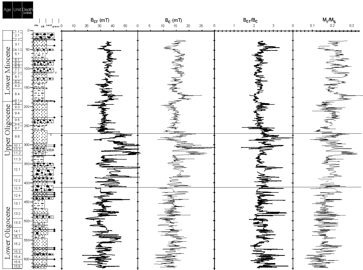
Fig. 2 – Down-core variation of the coercivity-dependent magnetic parameters ( B_{cr} and B_c ) and the inter-parametric hysteresis ratios B_{cr}/B_c and M_r/M_s for CRP-2/2A. The lines at 270 and 413 mbsf indicate the boundaries between intervals with different magnetic properties (see discussion in text, Fig. 1 & Tab. 1).
